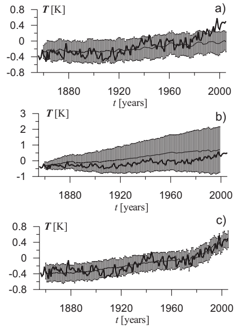
FIG. 7. The original GST values (the thick line) and 95% intervals for the bivariate models of GST: (a) a model (11) with solar activity fitted to the interval [1856–1985]; a model (12) with volcanic activity fitted to the interval [1856–1999]; (c) a model (13) with CO 2 atmospheric content fitted to the interval [1856–2005].
